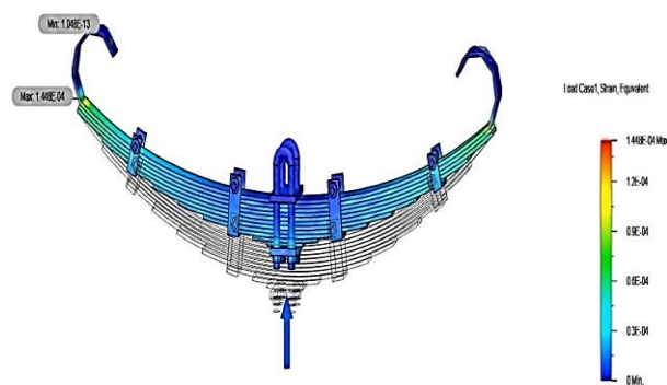
Fig. 17. Aluminium alloy strain distribution.
