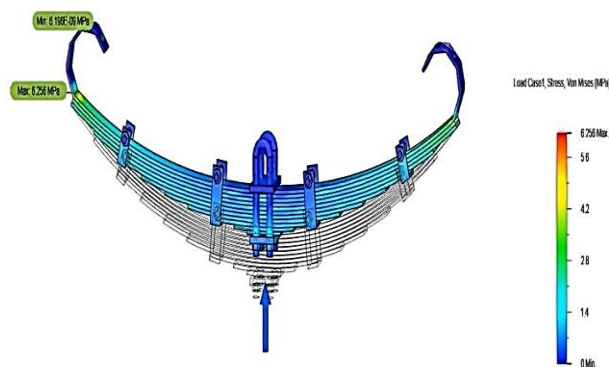
Fig. 16. Aluminium alloy stress concentration.
