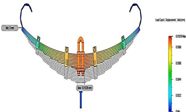
Fig. 15. Steel displacement distribution.
