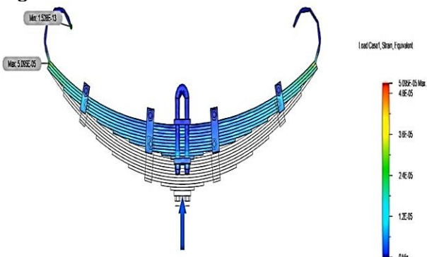
Fig. 14. Steel 7 strain distribution.
