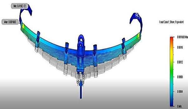
Fig. 23. Epoxy carbon Elastic Strain.
