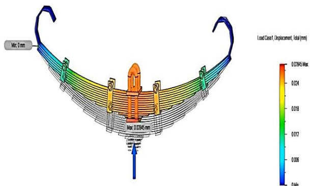
Fig. 18. Aluminum alloy displacement distribution.
